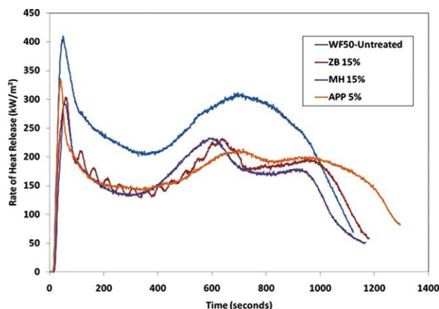
Figure 1 Examples of heat release rate curves for WF-50 untreated, WF-ZB 15%, WF-MH 15%, and WF-APP 5%. [Color figure can be viewed in the online issue, which is available at wileyonlinelibrary.com .]
