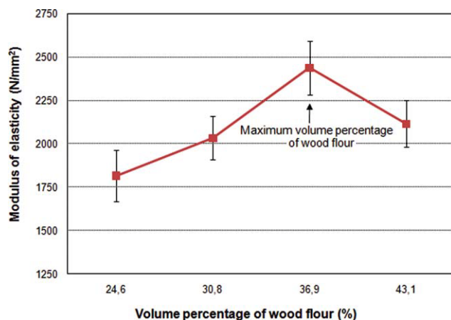
Figure 2 Modulus of elasticity of the WPCs without FR as a function of the volume percentage (%) of the WF. [Color figure can be viewed in the online issue, which is available at wileyonlinelibrary.com .]
